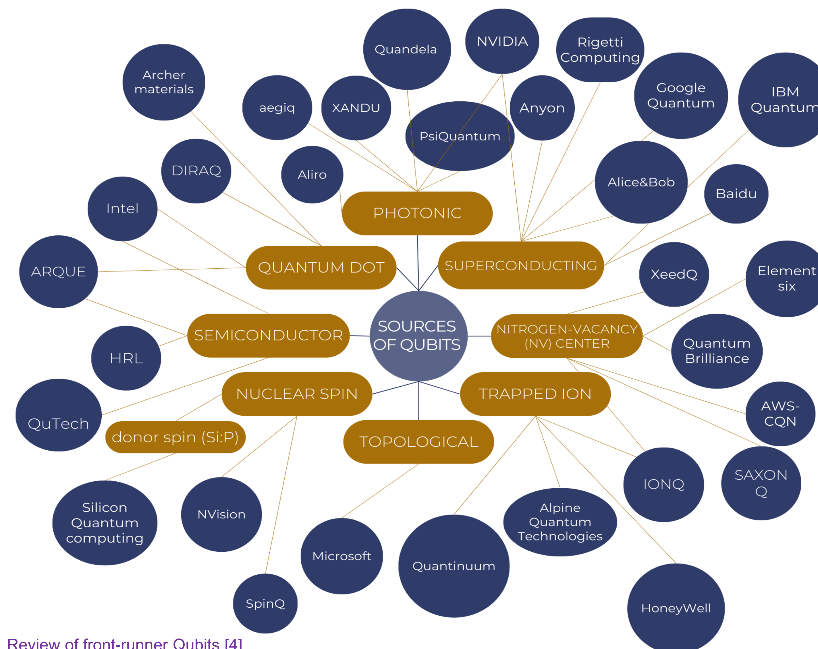
Review of front-runner Qubits [4].
