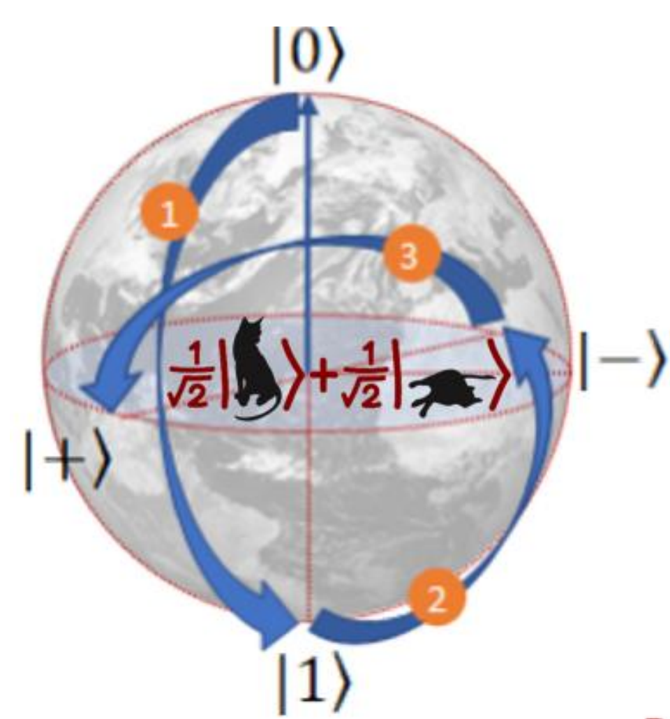
Bloch Sphere
