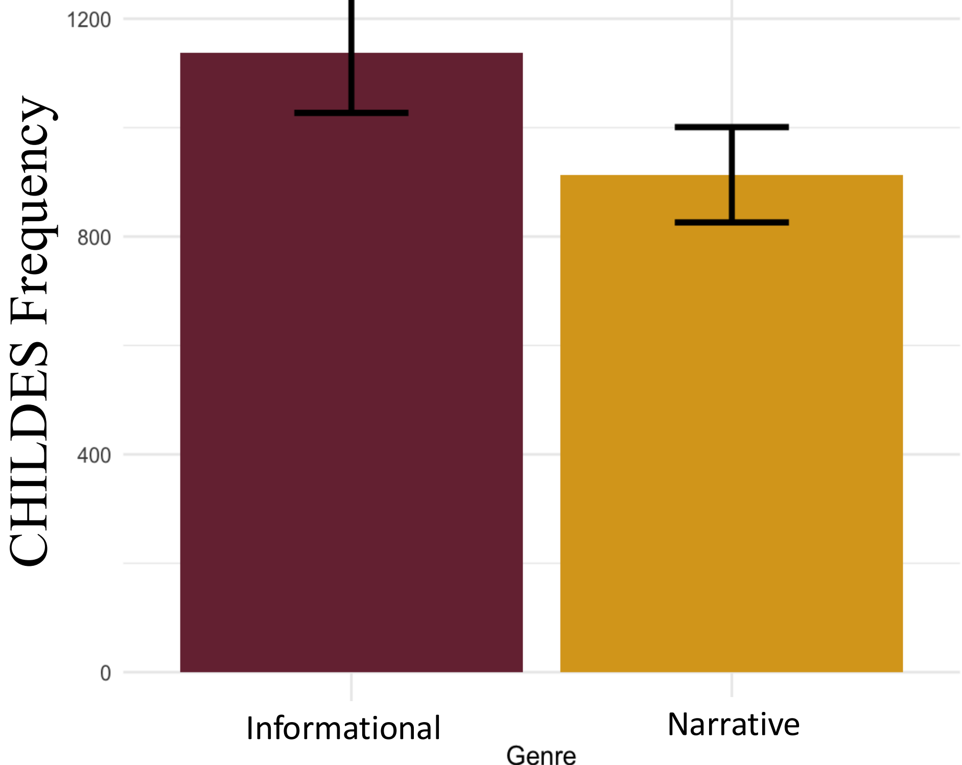
Figure 1: Bar graph of informational and narrative text frequency in child-directed speech. Bars are standard error of the mean.
