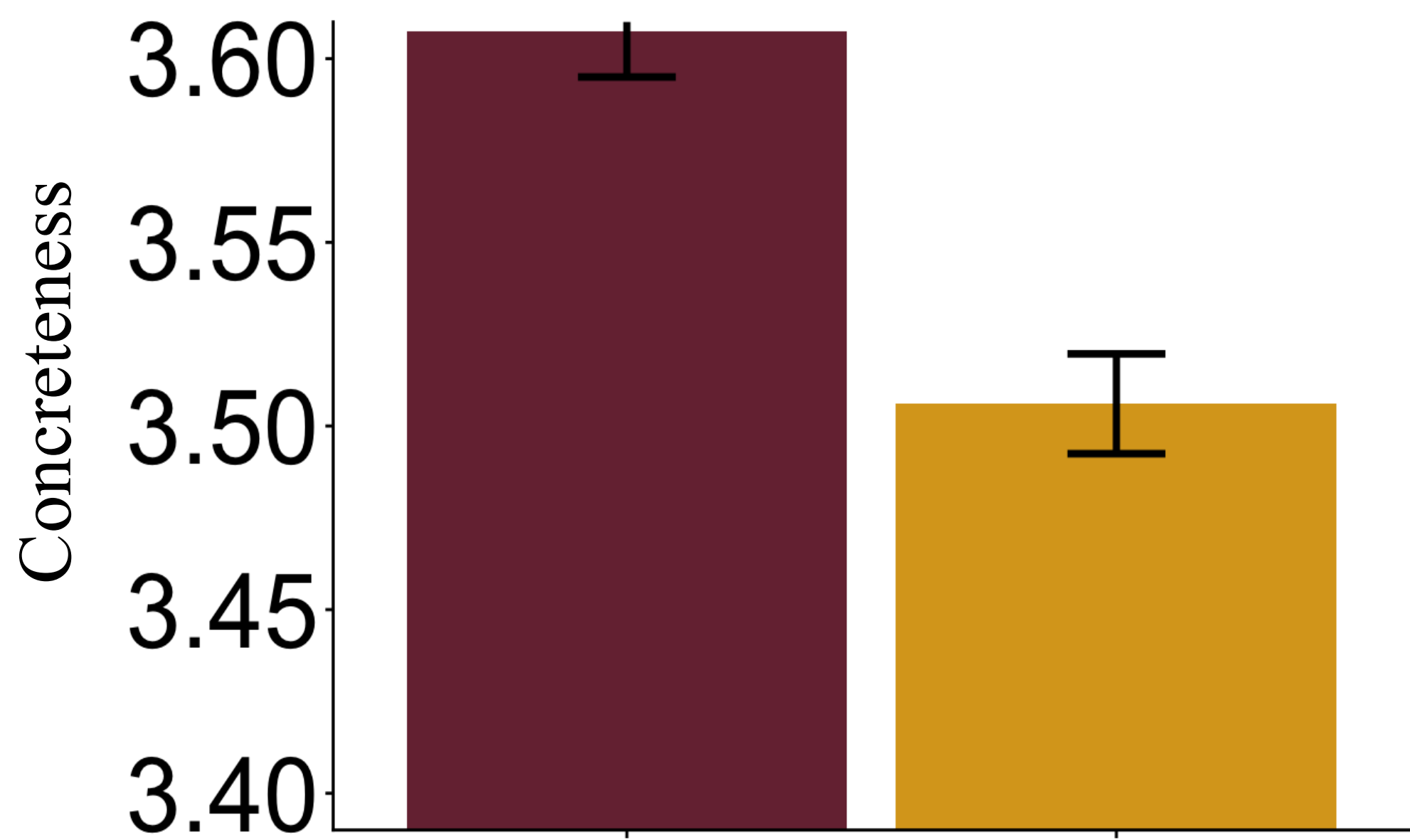
Figure 5: Bar graph of the mean concreteness of words across informational and narrative texts. Bars are standard error of the mean.
