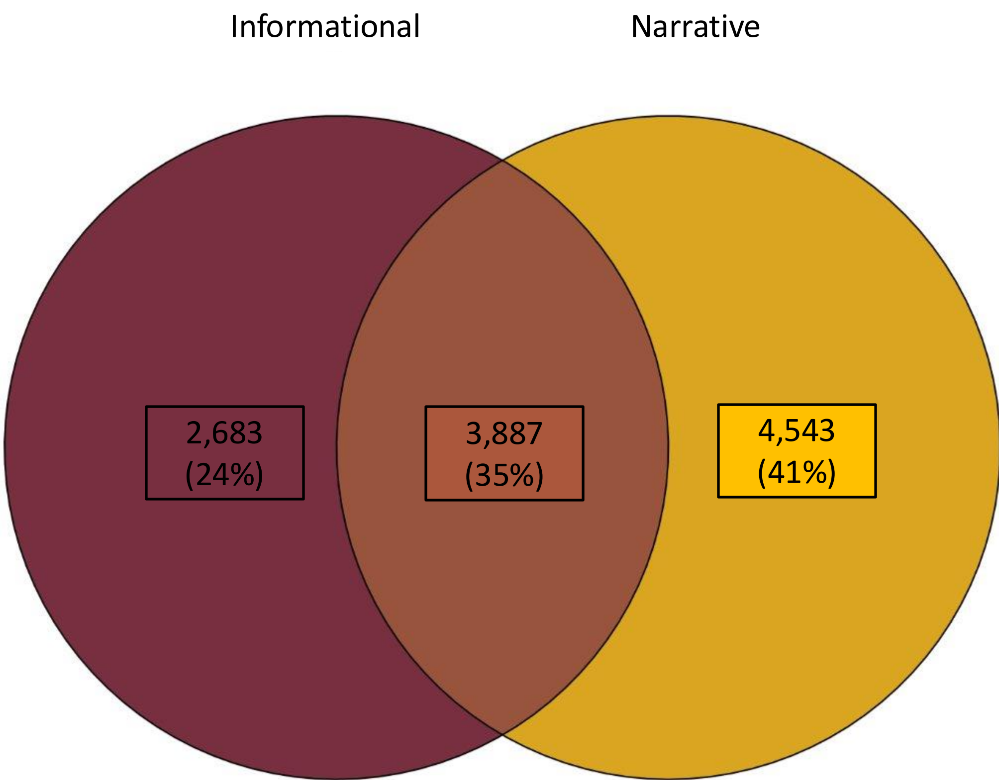
Figure 2: Venn Diagram displaying the distribution of unique words in informational and narrative texts.
